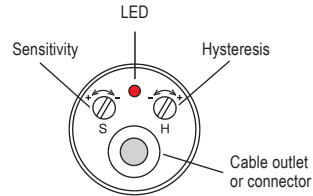
Fig. 18: Top view of level sensor
